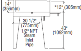
ER-12-5736 SIDE VIEW
