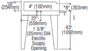
EP-EB-8-5736 SIDE VIEW
